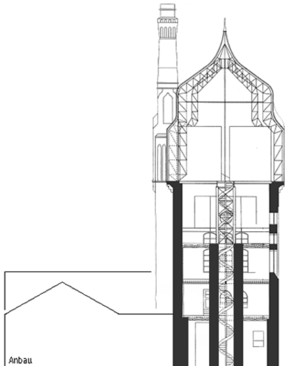
Schnitt West/Ost
